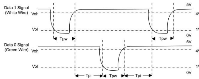
Figure1: Sequence Diagram
